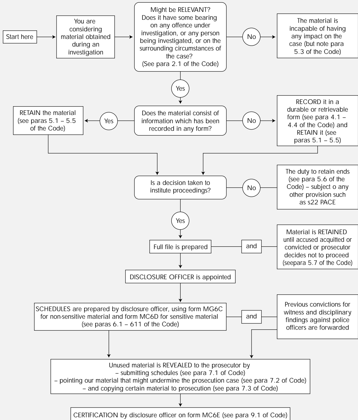
Flowchart 1
