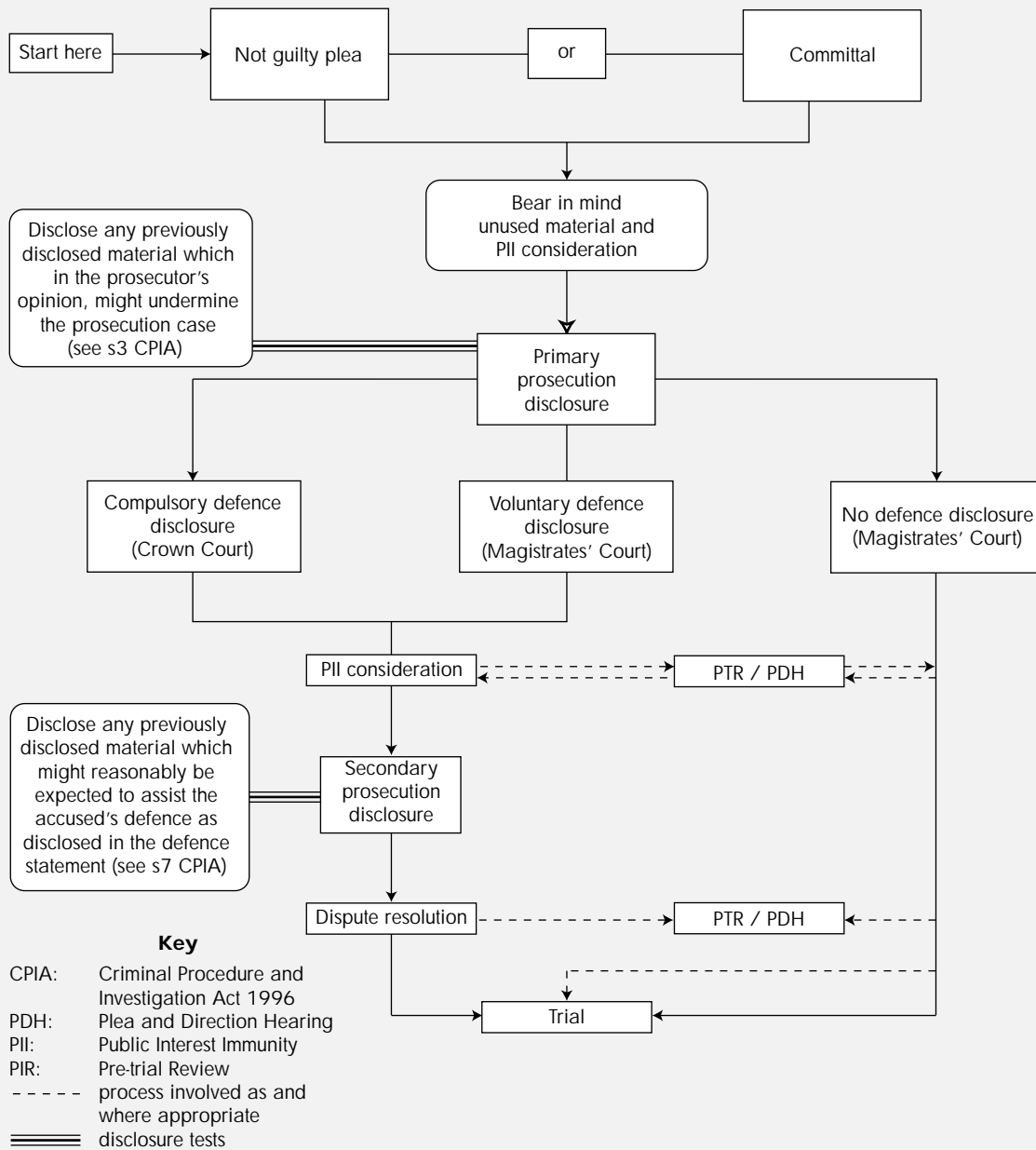
Flowchart 2
